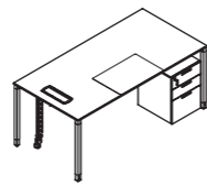
Model:RS-M1470 Sile:1400Wx700Dx750H Model:RS-M1680 Sile:1600Wx800Dx750H Model:RS-M1890 Sile:1800Wx900Dx750H
