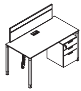
Model:RS-A1260 Sile:1200Wx600Dx750H Model:RS-A1470 Sile:1400Wx700Dx750H
